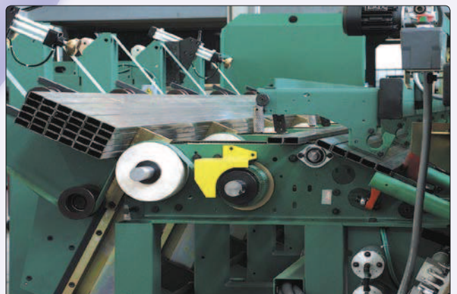
Device for layers loading of shaped profiles. It loads one complete layer at a time. Automatic pretension of belts included
