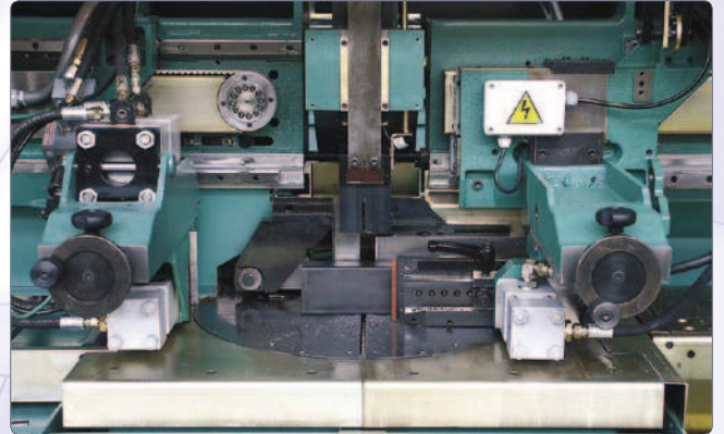
High speed automatic programmable loading, unloading and cutting table rotation
